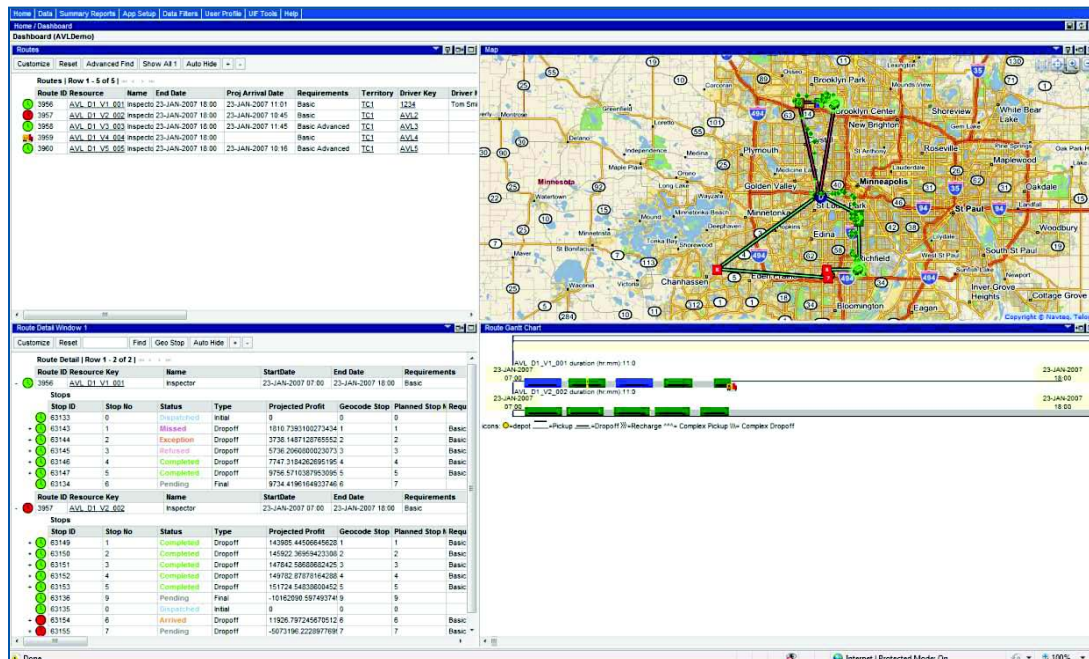
Figure 10: Route Planner with AVL Tracking
