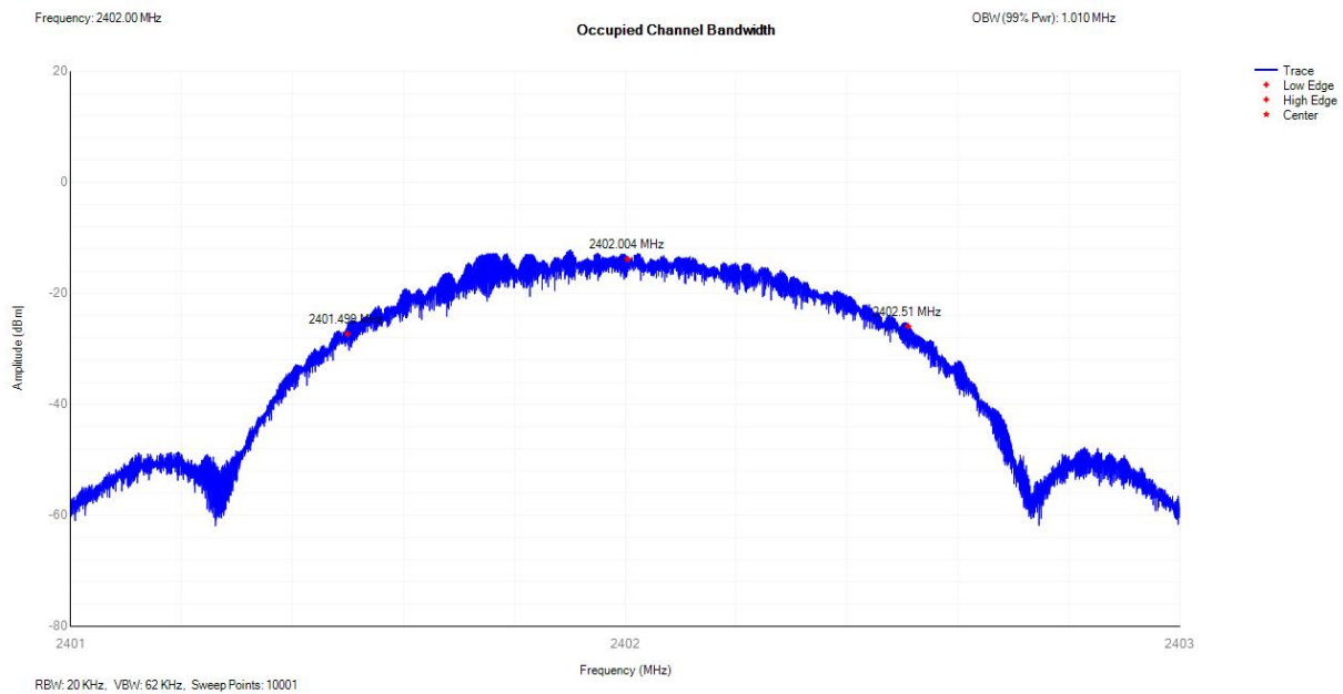
OBW NVNT BLE1M 2402MHz
